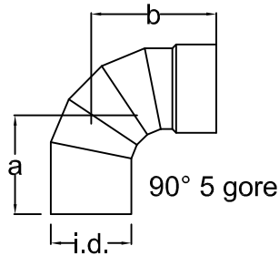
Duct Section
